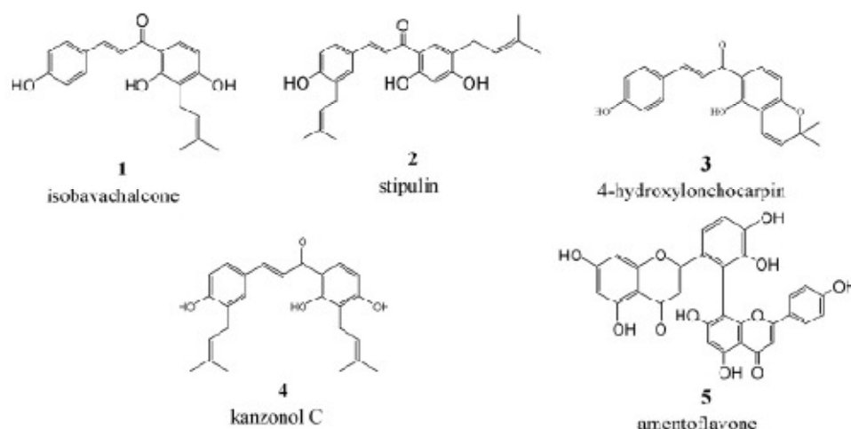
Fig. 1. Chemical structures of compounds isolated from the twigs of Dorstenia barteri Burau var. multiradiata .
