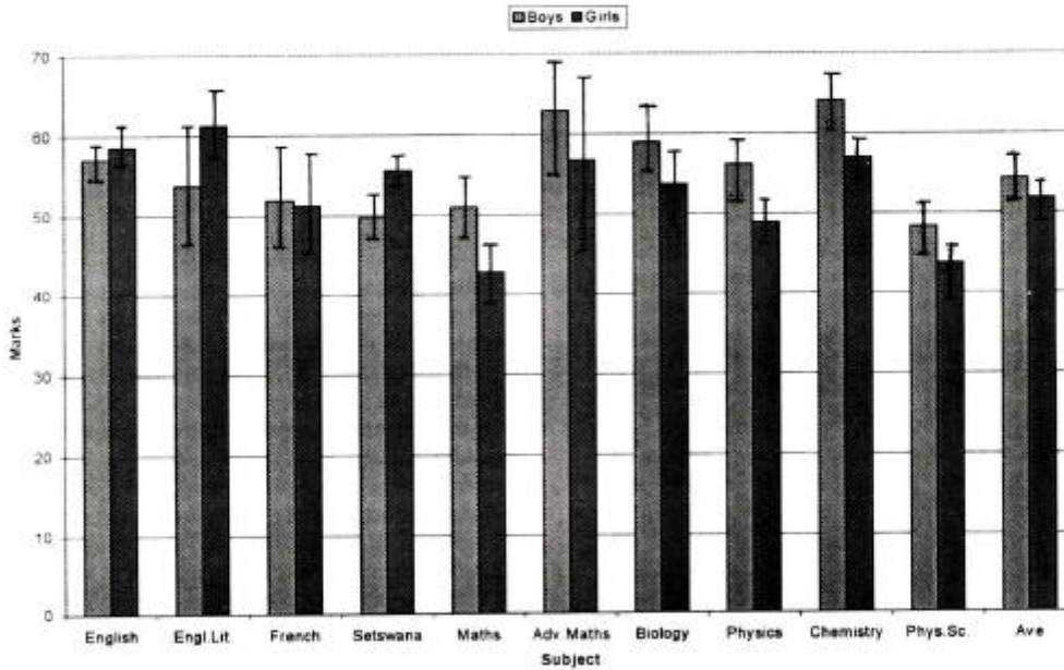
Fig.1 Mean marks and 95% confidence intervals for means per gender (marked by \bar{x} )
