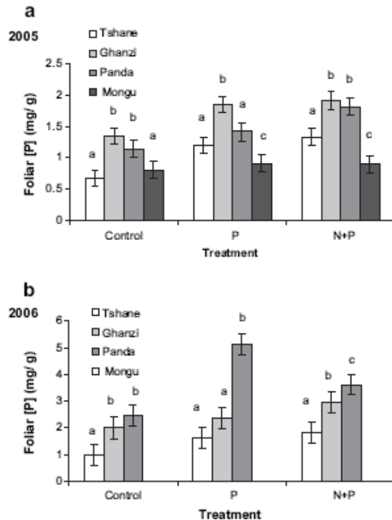
Fig. 4. Grass foliar phosphorus least square means at each site for each treatment (site by treatment interaction). Data are presented for year 1 (a) and year 2 (b). Sites vary in mean annual precipitation (Mongu = 879 mm, Pandamatenga = 698 mm, Ghanzi = 424 mm, Tshane = 365 mm). Nutrient treatments include increased phosphorus (P), increased nitrogen and phosphorus (N + P) and a control where no nutrients were added. Letters in both (a) and (b) denote significant Tukey Kramer adjusted differences between site means for each treatment. Data are missing for Mongu during year 2.
