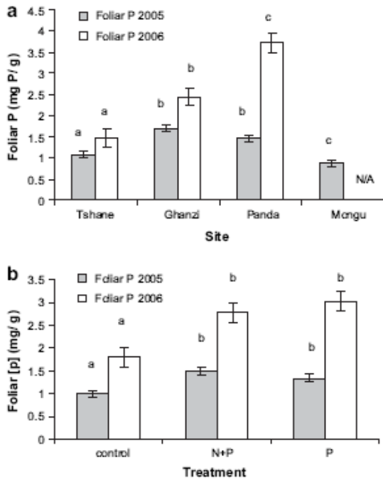
Fig. 3. Foliar grass phosphorus concentrations (mg P/g) least square means for year 1 (grey) and year 2 (white). Sites vary in mean annual precipitation (Mongu = 879 mm, Pandamatenga = 698 mm, Ghanzi = 424 mm, Tshane = 365 mm). Nutrient treatments include increased phosphorus (P), increased nitrogen and phosphorus (N + P) and a control where no nutrients were added. Letters in both (a) and (b) denote significant Tukey Kramer adjusted differences between site (Fig. a) and treatment (Fig. b) means. Data are unavailable for Mongu during year 2.
