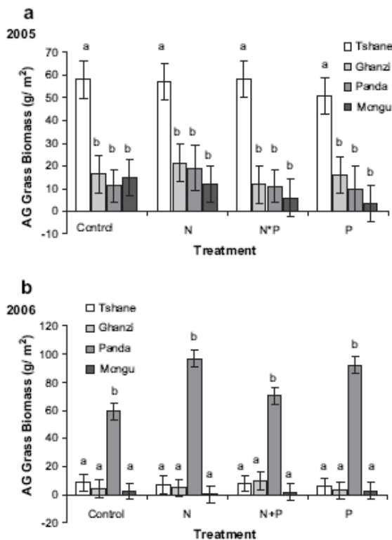
Fig. 6. Aboveground grass biomass ( \text{g}/\text{m}^2 ) least square means at each site for each treatment (site by treatment interaction). Data are presented for year 1 (a) and year 2 (b). Sites vary in mean annual precipitation (Mongu = 879 mm, Panda = 698 mm, Ghanzi = 424 mm, Tshane = 365 mm). Nutrient treatments include increased phosphorus (P), increased nitrogen and phosphorus (N+P) and a control where no nutrients were added. Letters in both (a) and (b) denote significant Tukey Kramer adjusted differences between site means for each treatment.
