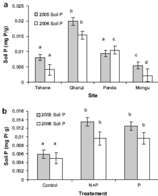
Fig. 1. Soil plant available phosphorus least square means for site effects (a) and treatment effects (b). Data are presented for year 1 (grey) and year 2 (white). Sites vary in mean annual precipitation (Mongu = 879 mm, Pandamatenga = 698 mm, Ghanzi = 424 mm, Tshane = 365 mm). Nutrient treatments include increased phosphorus (P), increased nitrogen and phosphorus (N + P) and a control where no nutrients were added. Letters in both (a) and (b) denote significant Tukey Kramer adjusted differences between site and treatment means, not between years.
