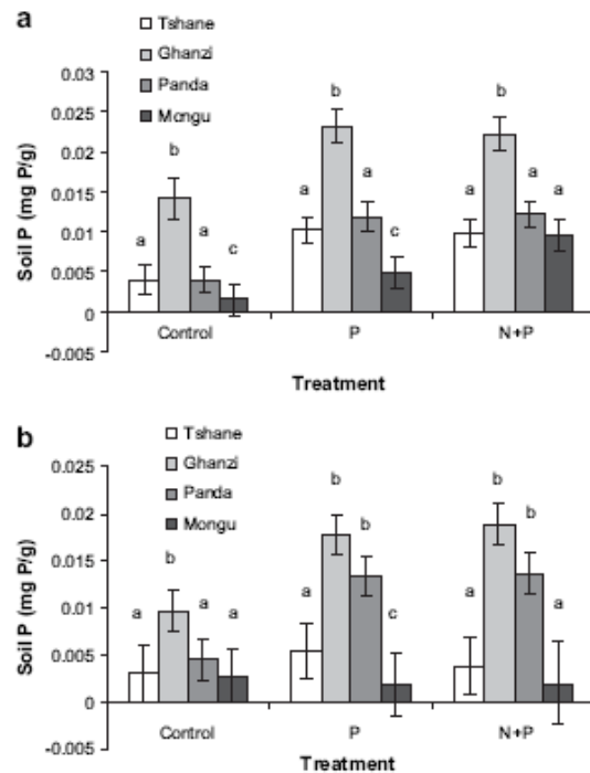
Fig. 2. Soil plant available phosphorus least square means at each site for each treatment (site by treatment interaction). Data are presented for year 1 (a) and year 2 (b). Sites vary in mean annual precipitation (Mongu = 879 mm, Pandamatenga = 698 mm, Ghanzi = 424 mm, Tshane = 365 mm). Nutrient treatments include increased phosphorus (P), increased nitrogen and phosphorus (N + P) and a control where no nutrients were added. Letters in both (a) and (b) denote significant Tukey Kramer adjusted differences between site means for each treatment.
